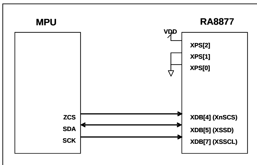
圖 7-7 : The MPU Interface Diagram of 3-Wire SPI
