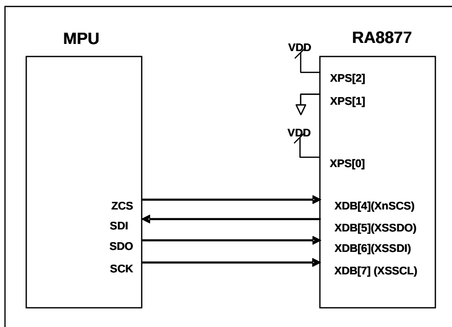
圖 7-13 : The MPU Interface Diagram of 4-Wire SPI
